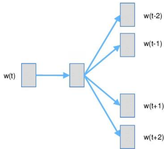
Figure 6.3: Skip-Gram Word Prediction
